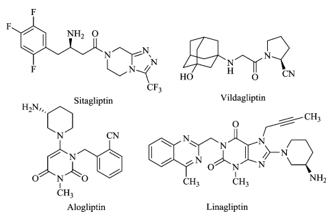
Figure 1. Marketed DPP-4 inhibitors.
