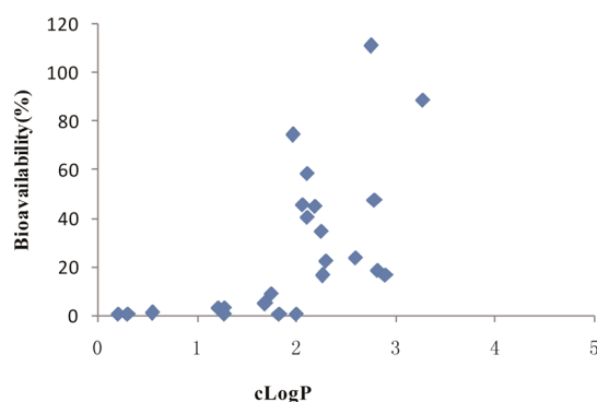
Figure 4. Bioavailability and cLogP.
