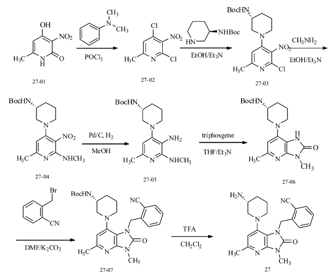
Scheme 1. Synthetic Route of Compound 27
