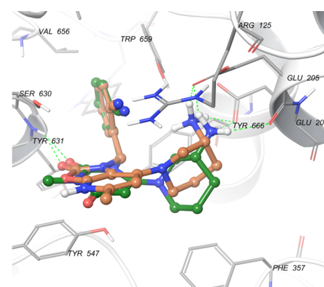
Figure 3. Superposed binding conformations of compound 27 (brown) and Alogliptin (dark green).
