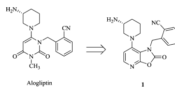
Figure 2. Scaffold-hopping leads to novel structure.
